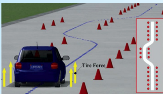
Vehicle Handling Test
